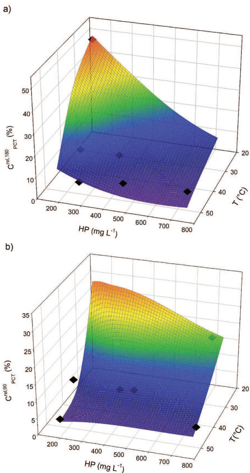
Fig. 3 Predicted (surfaces) and experimental (symbols) C_{PCT}^{rel,t} as a function of reaction temperature (T) and hydrogen peroxide concentration (HP). (a) F0 (t = 180 min); (b) F1 (t = 90 min)
