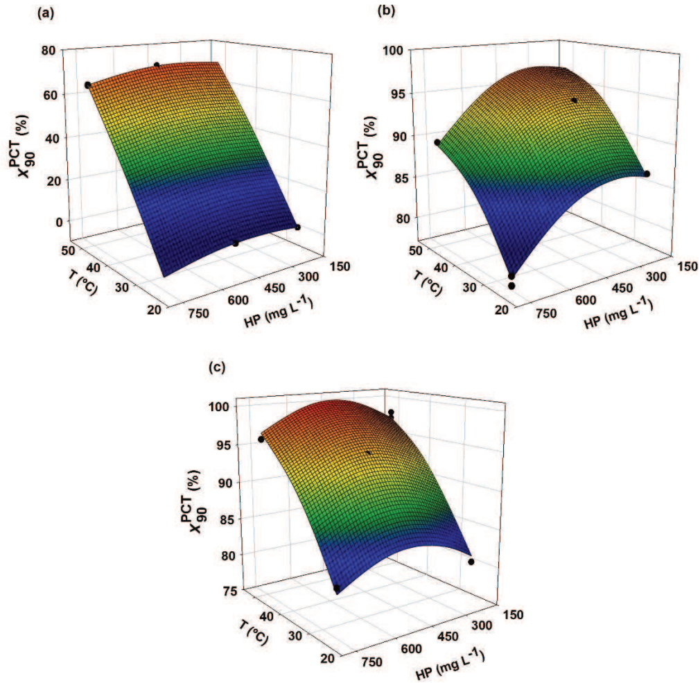
Fig. 3 Response surfaces and experimental values (circles) for X_{90}^{PCT} as a function of T and HP concentration. a) Dark conditions, b) Low Radiation, and c) High Radiation.
