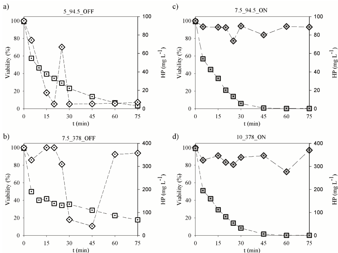
Figure 3 Cytotoxicity temporal evolution (diamond) and HP concentration (square). a) run #1: most adverse operational conditions for the reaction; b) run #3: Fenton reaction, medium [\text{Fe}^{2+}]^0 and high [\text{HP}]^0 operational conditions; c) run #7: photo-Fenton reaction, medium [\text{Fe}^{2+}]^0 and low [\text{HP}]^0 operational conditions; d) run #8: more favourable operational conditions for the reaction.
